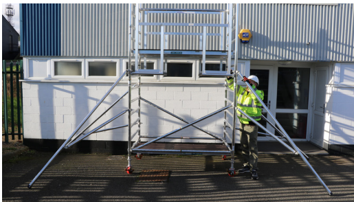
11. Fit 4 stabilisers at earliest opportunity keeping lower arms as horizontal as possible ideally 45 degrees. Stabilisers are fixed onto the frame uprights in each corner by the attached couplers.
