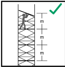
Platforms shall be installed with vertical distances between them not exceeding 2.1 m when assembling and dismantling except the distance to the first platform max 3.40m
