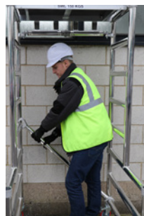
Fit a diagonal brace from the 1st to the 4th rung of the podium at the back of the unit.
